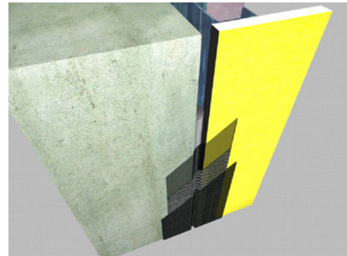
Recessed backer rod
