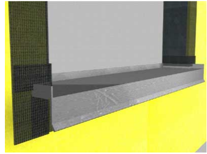
Apply AquaFlash System over vertical flashing legs.
