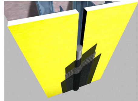
Projecting backer rod
