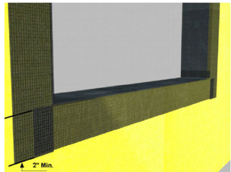
Overlap AquaFlash Mesh at least 51 mm (2 in).
