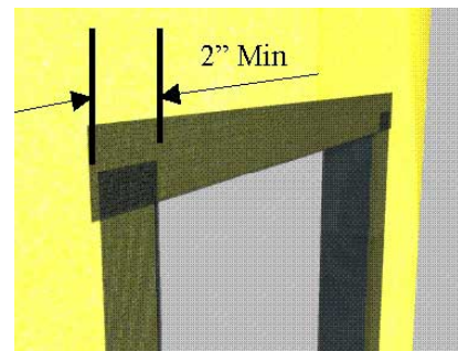
Overlap AquaFlash Mesh at least 51 mm (2 in).
